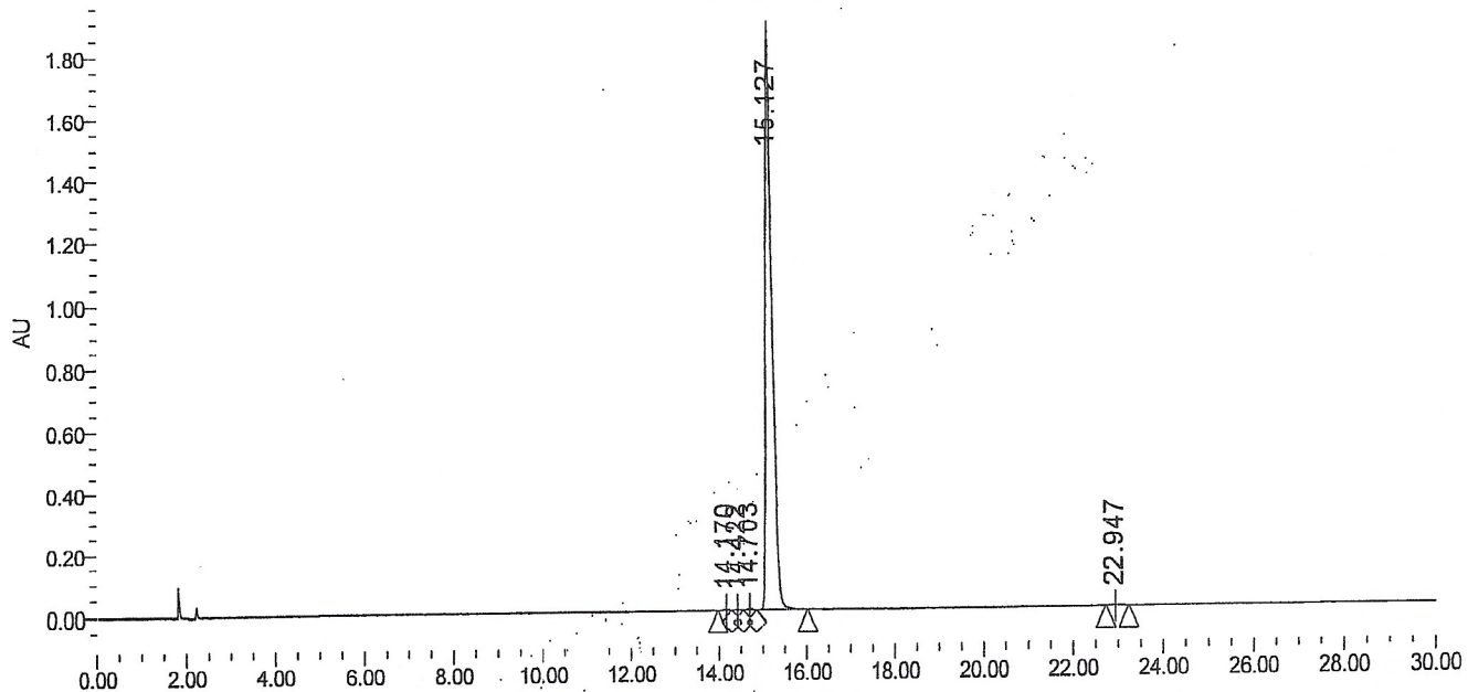
Auto-Scaled Chromatogram
